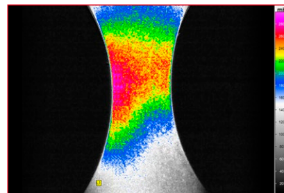
Thermal Stress Analysis with Lock-in Thermography
